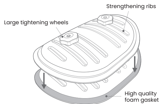
Curved Access Door
