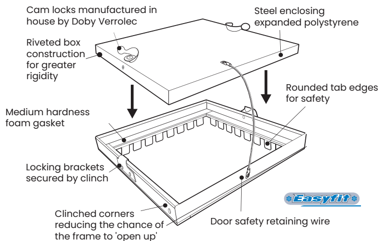
Tabbed Access Door – UK Made
